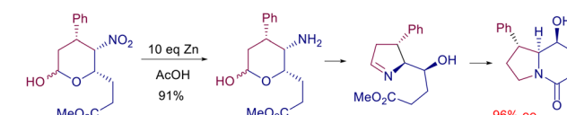
Scheme 14 Synthesis of nitrolactols and their application to the preparation of optically active indolizines.
