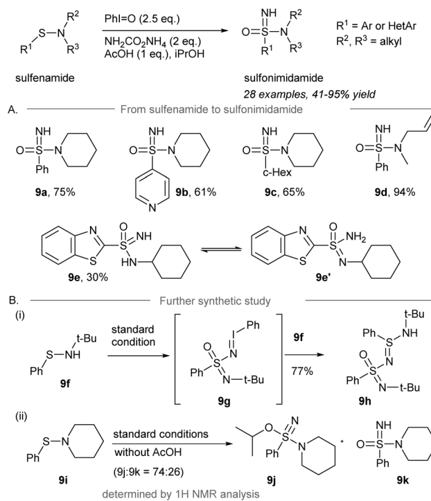
Scheme 7 Synthesis of sulfonimides from thiols through a one-pot \text{NH-} , \text{O-} , \text{RO-} transfer. 57
