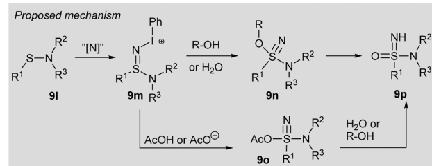
Scheme 9 (A) Synthesis of sulfonimidamides from sulfonamides through one-pot \text{NH-} and \text{O-} transfer. 58 (B) Further synthetic study of sulfonimidation.
