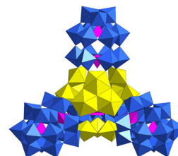
Fig. 3 View of [(\text{UO}_2)_{12}(\mu_3\text{-O})_4(\mu_2\text{-H}_2\text{O})_{12}(\text{P}_2\text{W}_{15}\text{O}_{56})_4]^{32-} . Color codes are the same as in Fig. 1.
