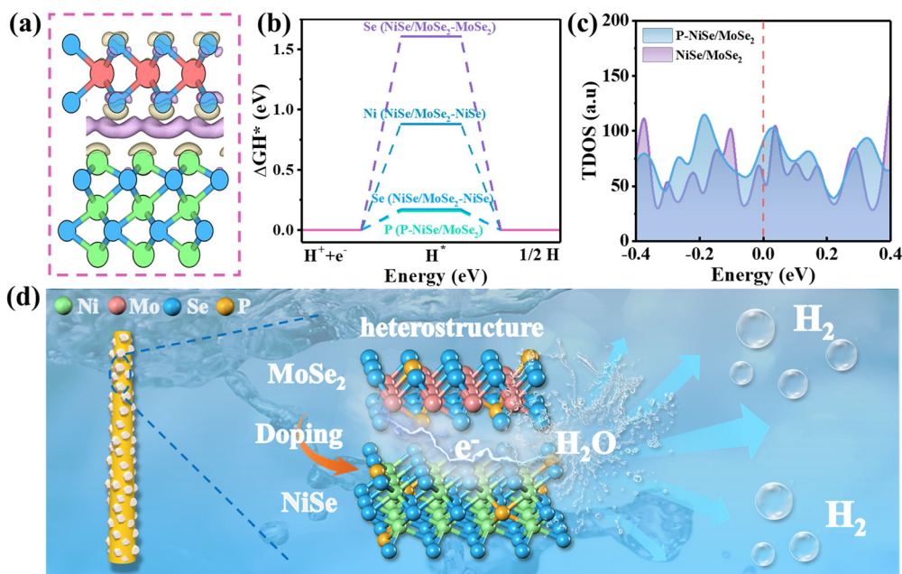
Fig. 6 (a) Charge density difference at the interface of the NiSe/MoSe 2 heterostructure. (b) Gibbs free-energy diagrams of NiSe/MoSe 2 and P-NiSe/MoSe 2 for H adsorption ( H^* ). (c) The calculated total electronic density of states (TDOS) of NiSe/MoSe 2 and P-NiSe/MoSe 2 . The Fermi level is set at 0 eV as a reference. (d) Hydrogen production from the P-NiSe/MoSe 2 @NF catalyst promoted by the comprehensive strategy of preparing a heterostructure and P doping.
