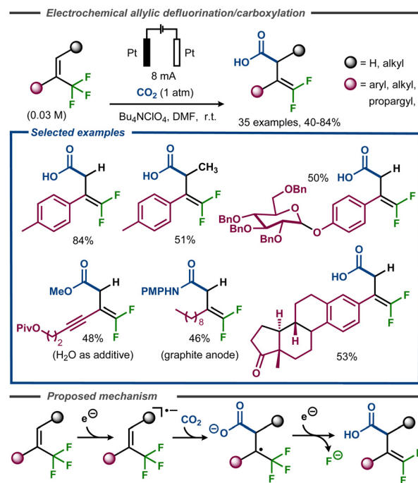
Fig. 17 Electroreductive formation of carboxylated gem -difluorostyrenes from \alpha,\alpha,\alpha -trifluoromethyl styrenes. 63
