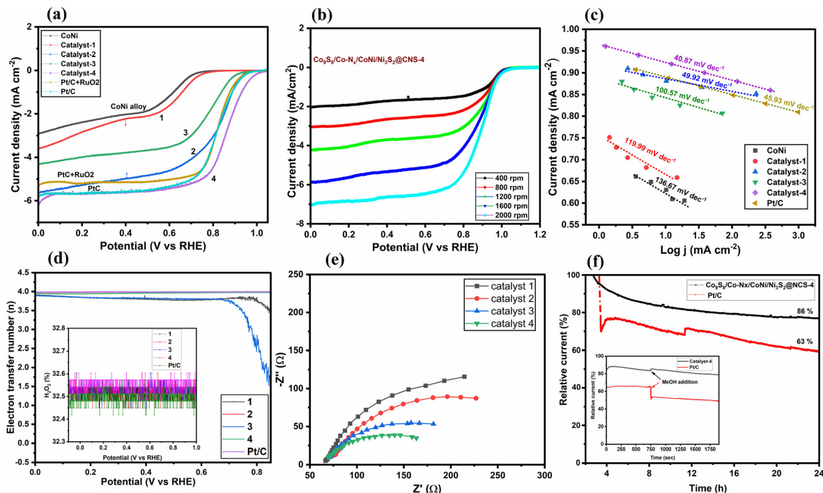
Fig. 6 Electrochemical ORR performances: (a) LSV curves of \text{CoS}/\text{Co}-\text{N}_x/\text{CoNi}/\text{Ni}_3\text{S}_2@ \text{CNS} 1-4 , commercial 20% Pt/C and Pt/C + \text{RuO}_2 in \text{O}_2 -saturated 0.1 M KOH, (b) LSV curves of \text{CoS}/\text{Co}-\text{N}_x/\text{CoNi}/\text{Ni}_3\text{S}_2@ \text{CNS}-4 , at various rotation rates, (c) Tafel plots of catalysts 1-4 and Pt/C, (d) Electron transfer number ( n ) of catalysts 1-4, and Pt/C, inset: the corresponding peroxide yields, (e) EIS spectra of catalysts 1-4, and (f) chronoamperometric responses of \text{Co}_9\text{S}_8/\text{Co}-\text{N}_x/\text{CoNi}/\text{Ni}_3\text{S}_2@ \text{CNS}-4 , and commercial 20% Pt/C in \text{O}_2 -saturated 0.1 M KOH solution at a rotation rate of 1600 rpm at \sim 0.4 V vs. RHE.
