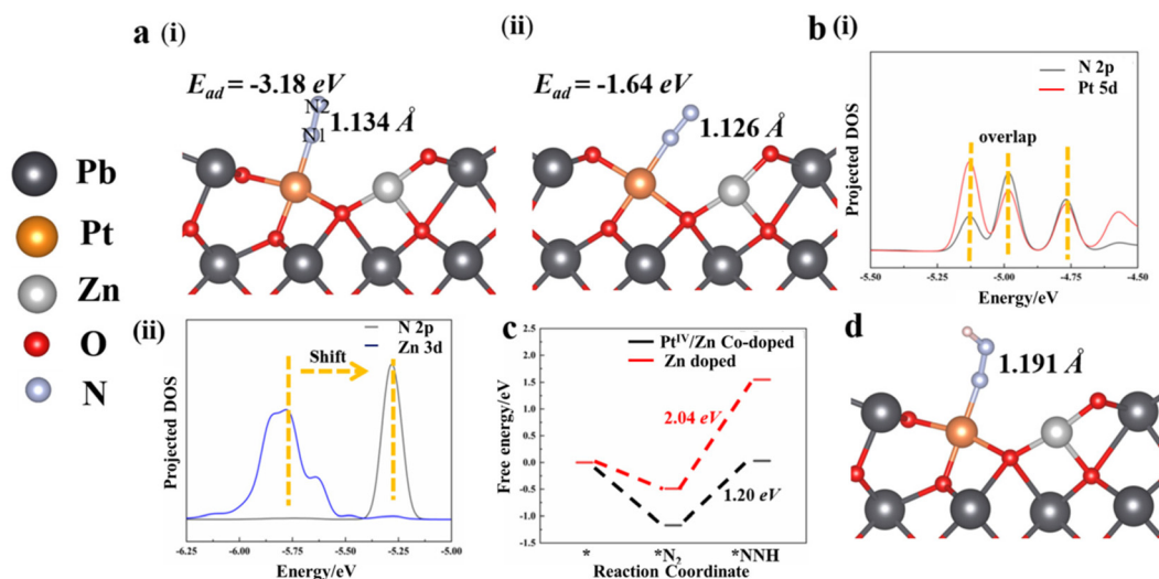
Fig. 8 (a) N_2 adsorbed on the (i) Pt^{IV} site and oxygen vacancy in the Zn/Pt^{IV} co-doped model with (ii) side-on configuration in the charged system. (b) Projected DOS of the (i) Zn/Pt co-doped and (ii) Zn -doped model. (c) Free energy profiles of the formation of *NNH in the Zn -doped and Zn/Pt^{IV} co-doped systems. (d) The optimized structure of *NNH adsorbed on the Zn/Pt^{IV} co-doped system.
