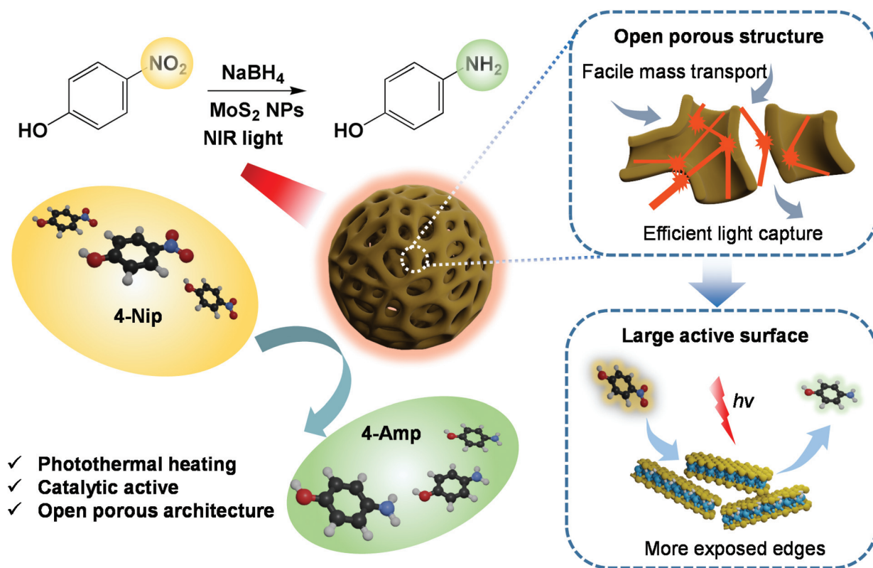
Scheme 2 Schematic of 4-Nip reduction with porous \text{MoS}_2 under NIR light illumination.
