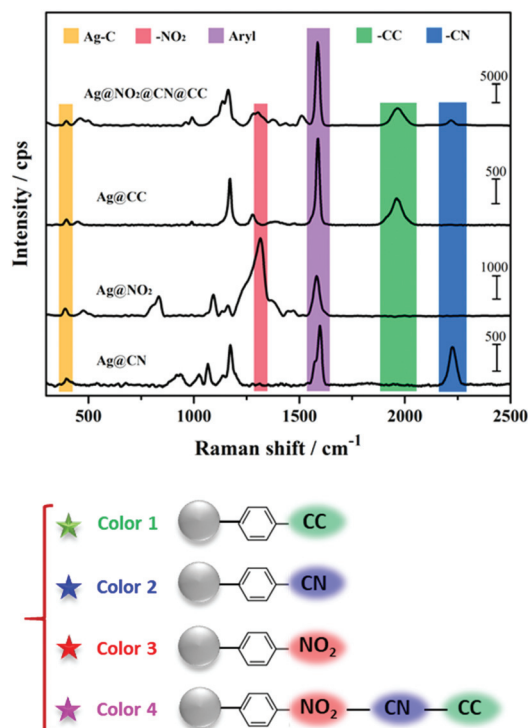
Fig. 5 SERS spectra of the three single layer-SERS tags and multilayer-coated \text{Ag@NO}_2\text{@CN@CCH} NPs. The excitation wavelength was 638 \text{ nm} , and the exposure time was 2 \text{ s} . The molecular structures of the three Raman reporters derived from aryl diazonium salts and the multilayer-coated \text{Ag@NO}_2\text{@CN@CCH} NPs are illustrated below.
