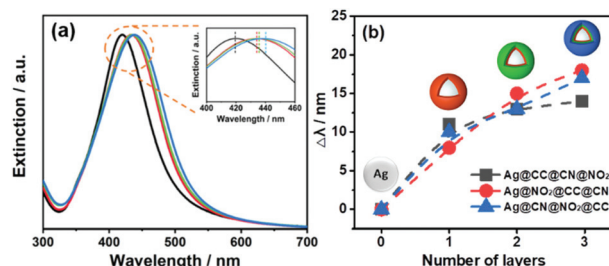
Fig. 3 (a) Normalized UV-vis spectra of Ag NPs (black line), \text{Ag@CN} (red line), \text{Ag@CN@NO}_2 (green line) and \text{Ag@CN@NO}_2\text{@CCH} (blue line); (b) Plot of \Delta\lambda (red shift of plasmon band) vs. the number of grafted layers around Ag cores for the step-by-step functionalization of \text{Ag@CCH@CN@NO}_2 , \text{Ag@NO}_2\text{@CCH@CN} and \text{Ag@CN@NO}_2\text{@CCH} .
