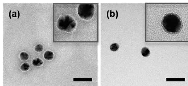
Fig. 2 Typical TEM images of (a) bare Ag NPs and (b) \text{Ag@NO}_2 . Scale bar = 50 nm. The insets show zoom of each figure to better observe the surface coating.
