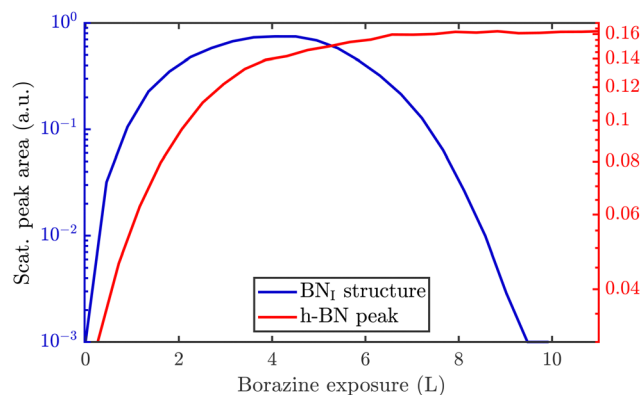
Fig. 3 In situ monitoring of the integrated peak intensities reveals that the \text{BN}_1 structure acts as precursor to the h-BN overlayer. The characteristic diffraction peaks for the \text{BN}_1 structure and the h-BN peak are plotted versus borazine exposure at a substrate temperature of 880 K. The \text{BN}_1 structure increases prior to the h-BN intensity and has already disappeared when the h-BN intensity exhibits its maximum.
