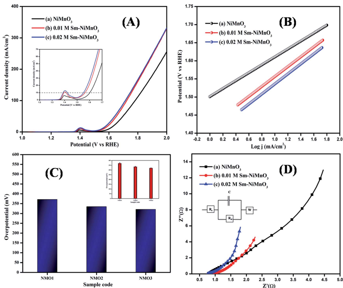
Fig. 5 (A) LSV spectra, (B) Tafel slope (C) Bar diagram (inset: error bar), and (D) EIS spectra of pristine \text{NiMnO}_3 , 0.01 M Sm-doped \text{NiMnO}_3 , and 0.02 M Sm-doped \text{NiMnO}_3 .
