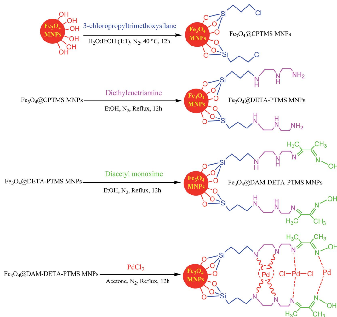
Fig. 1 Synthesis and structure of \text{Fe}_3\text{O}_4@\text{Pd-Schiff-base} MNPs. This figure was adapted with permission from Journal of Organometallic Chemistry , 2019, 880 , 196–212. 49
