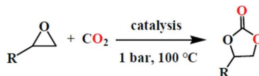
Scheme 6 The synthesis scheme for cycloaddition involving CO 2 . Reproduced with permission from ref. 22; copyright: 2020, ChemCatChem.
