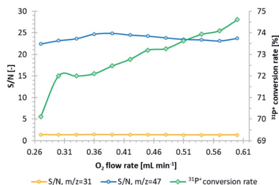
Fig. 1 Evaluation of the oxygen flow rate in CRC, based on S/N in the case of m/z equal to 31 (orange line) and 47 (blue line), and the estimation of the ^{31}\text{P}^+ \rightarrow ^{31}\text{P}^{16}\text{O}^+ conversion rate (green line).
