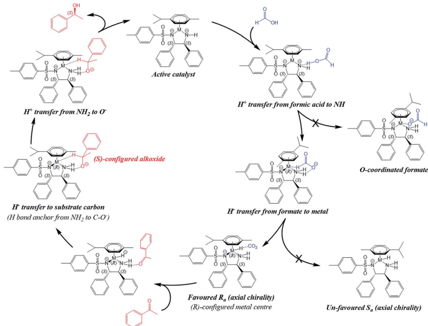
Fig. 12 The mechanism of asymmetric transfer hydrogenation catalysed by \text{Ru(II)} and \text{Os(II)} half-sandwich TsDPEN catalysts with formate as the hydride donor. The diamine ligand is always shown as (S,S) -configured. First, formic acid transfers \text{H}^+ to the catalyst \text{M}-\text{NH} , without prior formation of an \text{O} -coordinated intermediate. Hydride transfer then occurs from the formate anion to the metal, forming the hydride intermediate bearing a favoured (R) -configured metal centre and R_a axial chirality. The carbonyl of the substrate (acetophenone) forms a hydrogen bond with the catalyst \text{NH}_2 which serves to anchor the substrate molecule prior to the outer-sphere hydride transfer from \text{M}-\text{H} to the substrate carbon atom. After final \text{H}^+ transfer, the reduced substrate ( S -phenylethanol) is released, in turn regenerating the active 16-electron catalyst.
