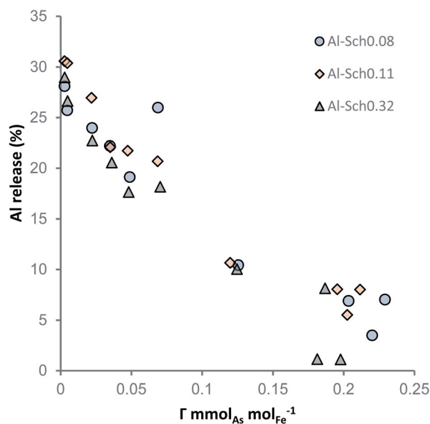
Fig. 4 Al released from Al-Sch after 72 h equilibration with the arsenate solution as a function of the adsorbed aqueous arsenate (mmol As 2 O 3 mol Fe -1 ).
