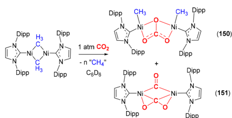
Scheme 44 Disproportionation transformations of the \text{CO}_2 moiety facilitated by a \text{Ni(I)} binuclear system.
