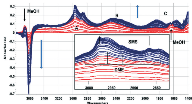
Fig. 2 Difference spectra recorded at 2 s intervals following the first 64 s after injecting an 8 \mu L pulse of \text{CH}_3\text{OH} into a SAPO-34 crystal at 523 K. The spectrum of the dehydrated SAPO-34 crystal has been subtracted from each spectrum. Colour change from red to blue after 20 s. Features specific to methanol present only during the first 20 s are marked. A, B, C refer to the \nu(\text{OH}) features of hydrogen bonded SAPO-34 acid sites. The inset shows an expansion of the \nu(\text{CH}) region, showing bands due to hydrogen bonded DME and SMS. Arrows indicate the direction of band intensity changes with time.
