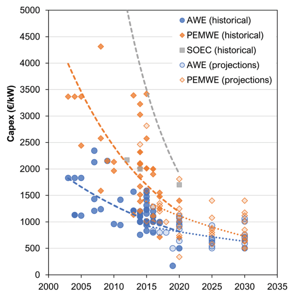
Fig. 158 Capex costs of electrolyser, both historical and projections for alkaline, PEM and SOEC technologies. Data compiled from ref. 1903–1906.
