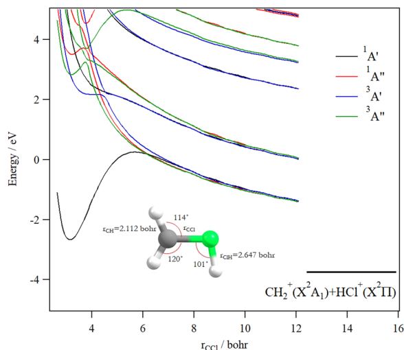
Fig. 8 spd(f) cc-pV5Z MRCI one-dimensional cuts of the PESs of the singlet and triplet states of \text{H}_2\text{CClH}_2^{2+} by lengthening the CCl distance ( r_{\text{CCl}} ). The r_{\text{CH}} distances are set to 2.112 bohr and the r_{\text{CH}} distance to 2.647 bohr, and the angles are set to their equilibrium values in \text{H}_2\text{CClH}_2^{2+} ground state. These curves are given relative to the \text{CH}_3\text{Cl}^{2+} ( X^3A_2 ) minimum energy.
