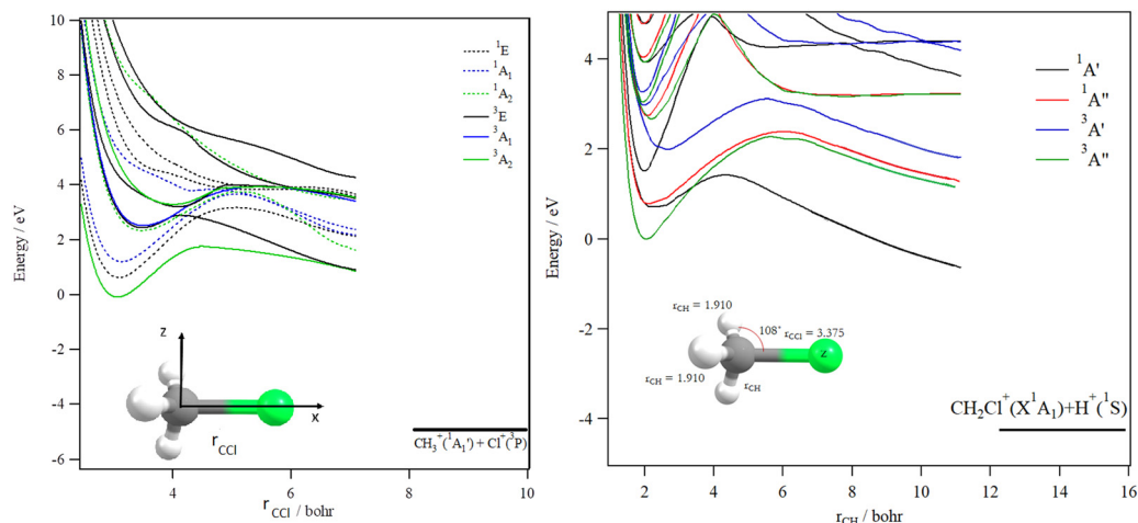
Fig. 7 spd(f) cc-pV5Z MRCI one-dimensional cuts of the PESs of the singlet and triplet states of \text{CH}_3\text{Cl}^{2+} lying in the 0–10 eV internal energy range. These curves are given relative to the \text{CH}_3\text{Cl}^{2+}(\text{X}^3\text{A}_2) minimum. Left: These curves are given as function of r_{\text{CCl}} which is the distance between the Cl atom and the C atom. r_{\text{CH}} (=2.084 bohr) and \theta_{\text{H-C-Cl}} (=116^\circ) are set to their equilibrium values in the neutral molecule. Right: These curves are obtained by lengthening one CH distance ( r_{\text{CH}} ). Remaining r_{\text{CH}} distances are set to 1.910 bohr) and CCl distance to 3.375 bohr, and \theta_{\text{H-C-Cl}} to 108^\circ ) i.e. their equilibrium values in \text{CH}_3\text{Cl}^{2+} ground state.
