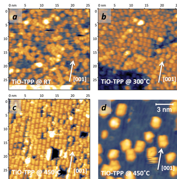
Fig. 23 STM images (W tip) of (a) 1 ML of \text{TiO} -TPP as deposited at RT, (b) after annealing to 300 ^\circ\text{C} and (c) 450 ^\circ\text{C} ; and (d) 0.2 ML of \text{TiO} -TPP after annealing to 450 ^\circ\text{C} .
