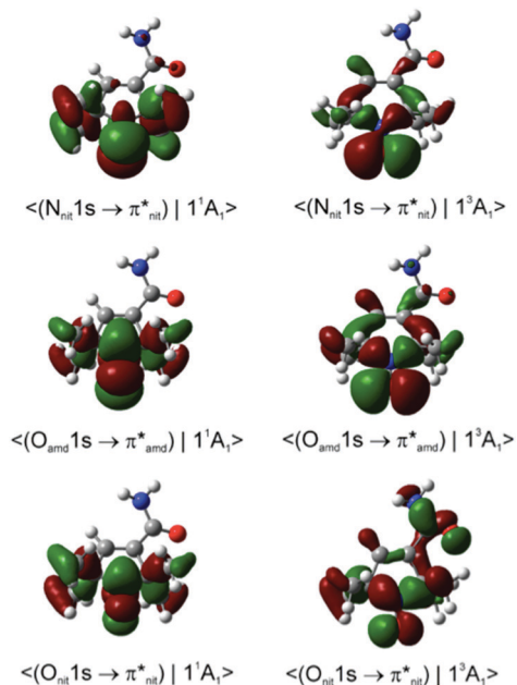
Fig. 8 Dyson spin orbitals of nit9 at the CAM-B3LYP//mixed level. The initial core-to-valence states concern the excitation from the 1s orbitals of amide (aml) or nitroxyl (nit) N or O atoms. The final states are the lowest singlet and triplet nit9 cations ( 1^1A_1 and 1^3A_1 ).
