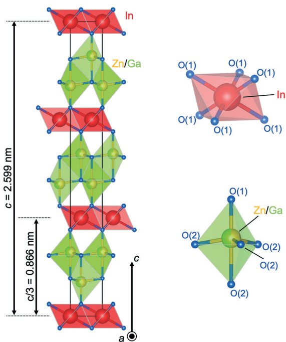
Fig. 5 Crystal structure of \text{InGaO}_3(\text{ZnO})_1 . Coordination of \text{InO}_6 is octahedra and \text{Zn/GaO}_4 is trigonal bipyramid. Because Zn and Ga cannot be separated, the Zn/Ga mixed site is referred to as the trigonal bipyramid in this paper.
