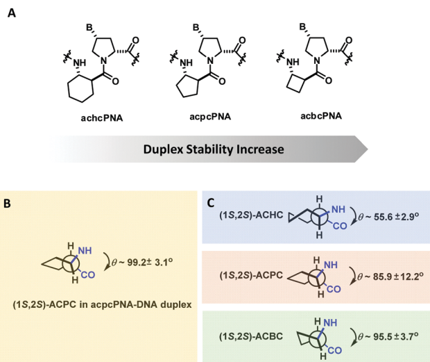
Fig. 27 (A) Structures of pyrrolidiny PNA homologs. (B) Torsional angle N(H)-C\alpha-C\beta-C(O) of (1S,2S)-ACPC in ACPC PNA. (C) Native torsional angles of cyclic \beta -amino acid oligomers are obtained from the literature (adapted with permission from ref. 137. Copyright 2012 American Chemical Society).
