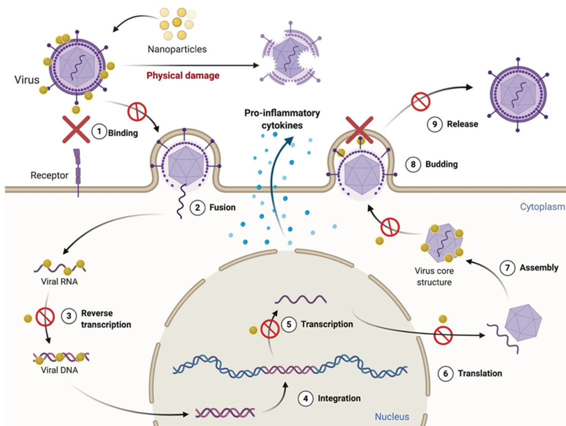
Fig. 7 Schematic showing the mechanism of antiviral action of OD nanoparticles.
