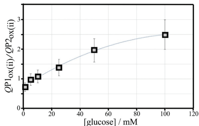
Fig. 10 Plot of the ratio of charges QP1_{ox}(ii)/QP2_{ox}(ii) versus glucose concentration for cyclic voltammetry experiments (scan rate 50 mV s -1 ; poly-NHG from 0.05 mM solution; 6 \mu g T1) in 0.1 M phosphate buffer pH 7. Polynomial line: -0.0001x^2 + 0.03x + 0.7649 ; errors estimated \pm 20\% .
