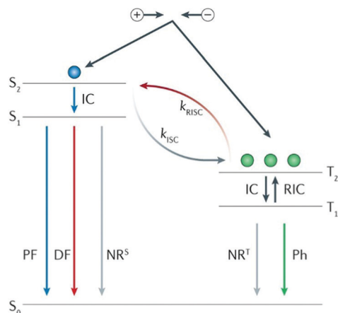
Fig. 4 Exciplex TADF luminescence mechanism. ISC, intersystem crossing; k_{ISC} , the rate constant of ISC; k_{RISC} , the rate constant of endothermic RISC; NR^S , singlet nonradiative decay; NR^T , triplet nonradiative decay; and RIC, reverse internal conversion. Reprinted with permission from ref. 40. Copyright © 2018, Macmillan Publishers Limited.
