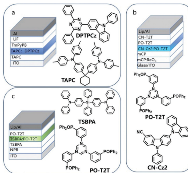
Fig. 10 Example of blending a donor and acceptor to adjust the emission color of OLED. (a) Blue: TAPC:DTPPCz. (b) Cyan: PO-T2T:CN-Cz2. (c) Green: PO-T2T:TSBPA.
