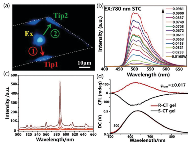
Fig. 7 (a) PL microscopy image of BTC under excitation. Reprinted with permission from ref. 54. Copyright © 2015 Wiley-VCH Verlag GmbH & Co. KGaA, Weinheim. (b) The up-conversion PL spectra of STC cocrystals. Reprinted with permission from ref. 55. Copyright © 2017 Wiley-VCH Verlag GmbH & Co. KGaA, Weinheim. (c) PL spectra of CBP@TCNB (1:1) as a function of the pump laser energy. Reprinted with permission from ref. 56. Copyright © 2018, American Chemical Society. (d) Circularly polarized luminescence spectra of a cast film of R -Py/TCNB CT complexes excited by 360 nm. Reprinted with permission from ref. 57. Copyright © 2019 Wiley-VCH Verlag GmbH & Co. KGaA, Weinheim.
