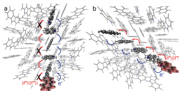
Fig. 4 Schematic representation of two possible exciton transport pathways involving dimers A and B (a), or dimer C (b). The highlighted molecule represents the initial position for electron ( e^- , in blue) or exciton ( |S^*\rangle or |T^*\rangle ) transport (in red). The crosses indicate specific pathways that are less likely due to the small values of the couplings.
