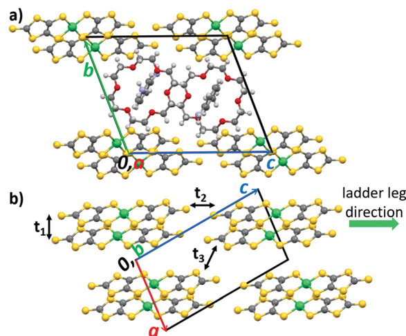
Fig. 16 Crystal structure of (HMPD)[(18)crown-6][Ni(dmit) 2 ] (16). (a) Unit cell viewed along the a axis. (b) [Ni(dmit) 2 ] − anion arrangement within the ac plane. Three types of intermolecular interactions ( t_1 – t_3 ) were observed. 61
