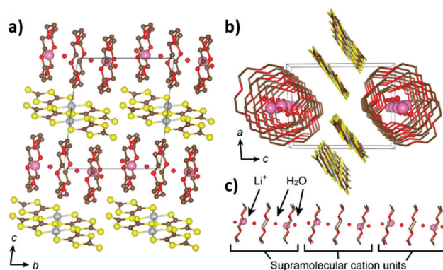
Fig. 17 Crystal structures of salt Li 2 [(18)crown-6] 3 [Ni(dmit) 2 ] 2 (H 2 O) 4 (17) viewed along the (a) a axis and (b) b axis. (c) Arrangement of supramolecular cation units ((18)crown-6, Li + , and water molecules) that adopt an ion channel configuration. Reproduced with permission from ref. 64. Copyright 2018 American Chemical Society.
