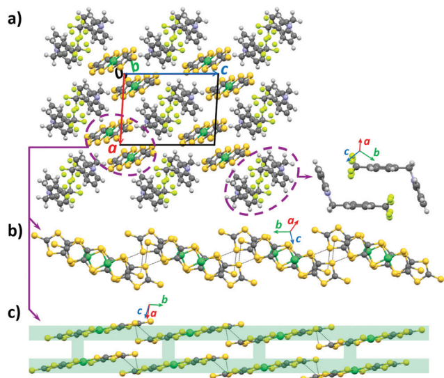
Fig. 15 Crystal structure of [4'-CF 3 -BzPy][Ni(dmit) 2 ] (13). (a) Viewed along b axis which shows a chair type cation dimer. (b) Anion chain formed via lateral-to-lateral S...S contacts and (c) anion ladder type with a representation of the ladder legs and rungs. 59
