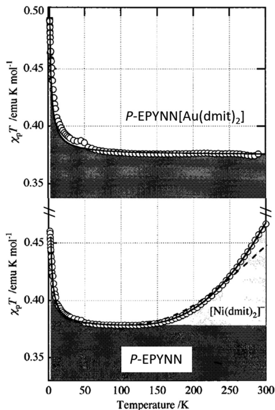
Fig. 14 Temperature dependence of the paramagnetic susceptibility ( \chi_p ) of p -EPYNN[Au(dmit) 2 ] (top) and p -EPYNN[Ni(dmit) 2 ] (12) (bottom). The solid lines are the theoretical fit using equations in the text. The thick and bright regions in the bottom represent the contribution from p -EPYNN and Ni(dmit) 2 , respectively. The broken line in bottom is the trial best fit using a simple dimer model. Adapted with permission from ref. 57. Copyright 1999 American Chemical Society.
