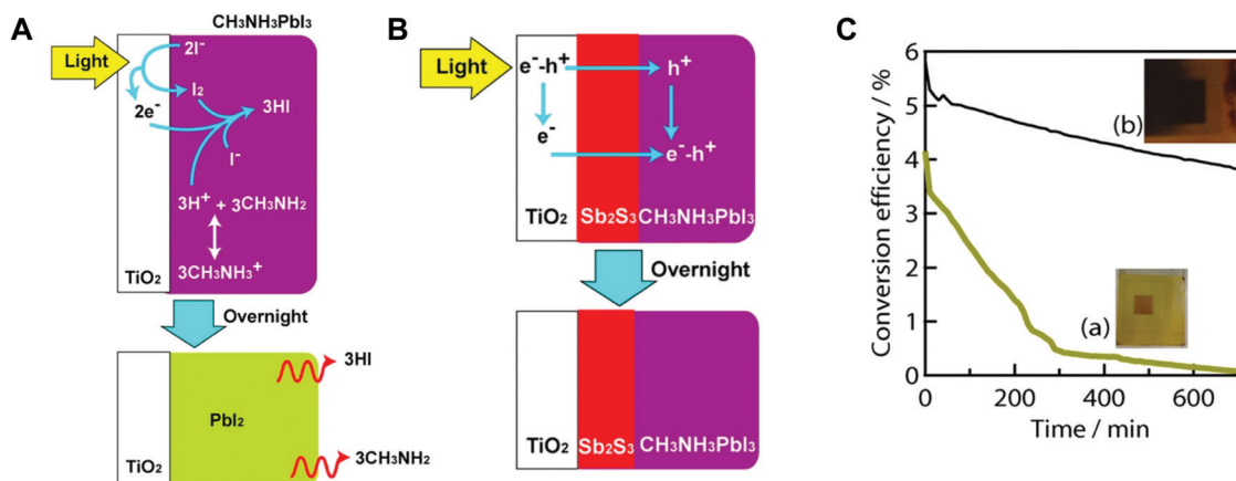
Fig. 8 A schematic illustrating the UV-induced degradation of MAPbI 3 at the TiO 2 interface (A). Protection against UV light degradation in a PSC containing an antimony trisulfide (Sb 2 S 3 ) layer between the mesoporous TiO 2 and the perovskite absorber. PCE retainment of an unmodified and unencapsulated methylammonium lead iodide PSC (A) vs. an antimony trisulfide modified PSC (B) under UV light with an intensity of 100 mW cm -2 for 12 hours. Photographs of the device showing PbI 2 discoloration in the unmodified PSC are included (C). Reproduced with permission from ref. 50. Copyright 2014 American Chemical Society.
