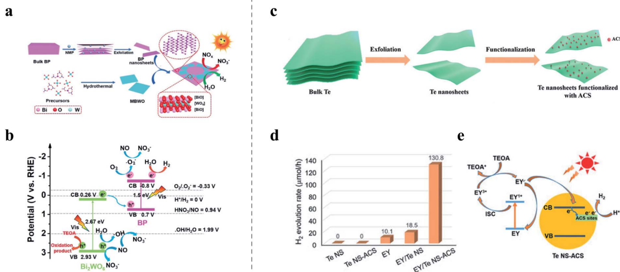
Fig. 9 (a and b) Photocatalytic NO removal based on the composite film of BP/monolayer \text{Bi}_2\text{WO}_6 . 209 (a) schematic illustration of the synthesis of the BP/monolayer \text{Bi}_2\text{WO}_6 heterojunction; (b) mechanism of photocatalytic NO removal and water splitting based on the BP/monolayer \text{Bi}_2\text{WO}_6 heterojunction under visible-light irradiation, showing the various redox potentials versus RHE. (c–e) Photocatalytic \text{H}_2 evolution based on atomic cobalt species (ACS) functionalized tellurene nanosheets (Te NS-ACS). 210 (c) illustration of the synthesis of Te NS-ACS; (d) the photocatalytic \text{H}_2 evolution activities of pure tellurene nanosheets (Te NS) with and without ACS functionalization and Eosin Y (EY) as a light absorber under visible light; (e) mechanism of the photocatalytic \text{H}_2 evolution based on Te NS-ACS. (a and b) Reproduced with permission, 209 Wiley-VCH. (c–e) Reproduced with permission, 210 Wiley-VCH.
