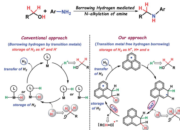
Scheme 1 Alkylation of amines by alcohols via hydrogen borrowing: conventional approach and our strategy.
