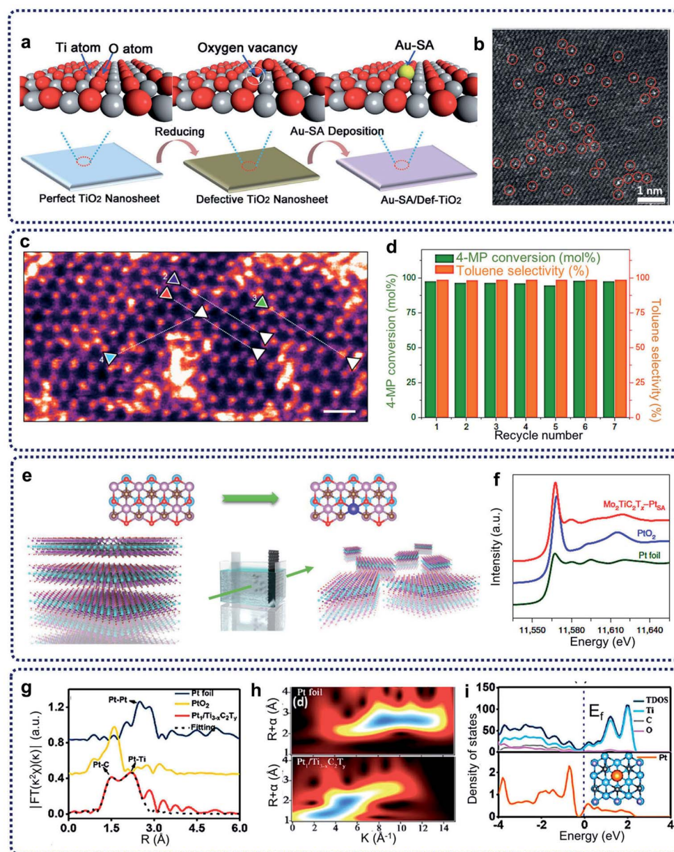
Fig. 3 (a) Schematic illustration of the synthesis procedure and the results of Au-SACs/Def-TiO 2 . (b) HAADF-STEM image, single atomic Au sites highlighted by red circles. Reproduced by permission. 32 Copyright 2018, Wiley-VCH. (c) HAADF image of the basal plane of Co-SMoS 2 (post-catalysis). Scale bar, 0.5 nm. (d) Stability test of Co-SMoS 2 for HDO of 4-methylphenol. Reaction conditions: 3 MPa at 180 °C. Reproduced by permission. 33 Copyright 2017, Springer Nature. (e) Schematic of the electrochemical exfoliation process of MXene with immobilized single Pt atoms. (f) Normalized XANES spectra at the Pt L 3 -edge of the Pt foil, PtO 2 and Mo 2 TiC 2 T x -PtSA. Reproduced by permission. 34 Copyright 2018, Springer Nature. (g) EXAFS FT k^2 -weighted \chi(k) function spectra of Pt 1 /Ti 3-x C 2 T y and Pt foil. (h) WT for the k^2 -weighted Pt L 3 -edge EXAFS signals in Pt 1 /Ti 3-x C 2 T y and Pt foil. (i) TDOS and PDOS of Pt 1 /Ti 3-x C 2 T y . Inset: schematic model. Reproduced by permission. 35 Copyright 2019, American Chemical Society.
