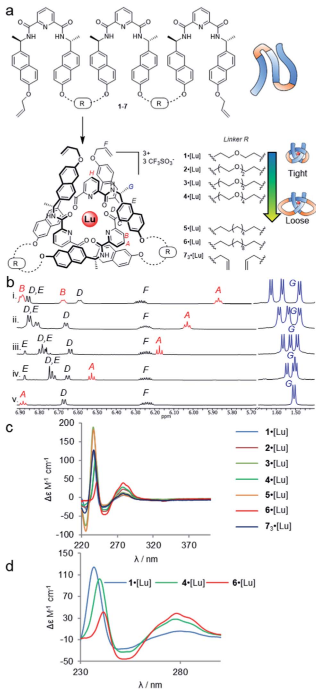
Fig. 2 Effects of entanglement tightness in overhand knots. (a) Structure of knots 1–6 ·[Lu] and circular helicate 73 ·[Lu]. Reagents and conditions: \text{Lu}(\text{CF}_3\text{SO}_3)_3 , MeCN, 80 °C, 16–24 h. (b) Partial ^1\text{H} NMR spectra (600 MHz, 298 K, MeCN- d_3 ) of overhand knots and helicates (i) 1 ·[Lu], (ii) 2 ·[Lu], (iii) 3 ·[Lu], (iv) 4 ·[Lu] and (v) 73 ·[Lu]. For full spectral assignments, see ESI† (c) Overlaid circular dichroism spectra of overhand knots 1–6 ·[Lu] and circular helicate 73 ·[Lu] (MeCN), normalised for absorbance. (d) Expanded region of CD spectra of 1 ·[Lu], 4 ·[Lu] and 6 ·[Lu], showing correlations between chiral expression and tightness of the core entanglement around the lanthanide ion.
