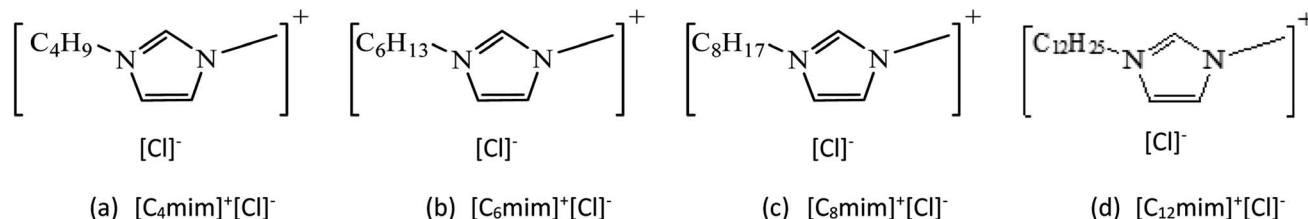
Fig. 1 Chemical structure of the used ILs molecules.
