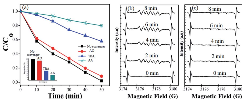
Fig. 8 (a) Effects of different radical scavengers on CV degradation over 1T-MoS 2 @(Bi 0.40 Fe 0.60 )VO 4 under visible light irradiation. (b) DMPO spin trapping EPR spectra for DMPO- • O 2 - and (c) DMPO- • OH - under visible light over 1T-MoS 2 @(Bi 0.40 Fe 0.60 )VO 4 photocatalyst.
