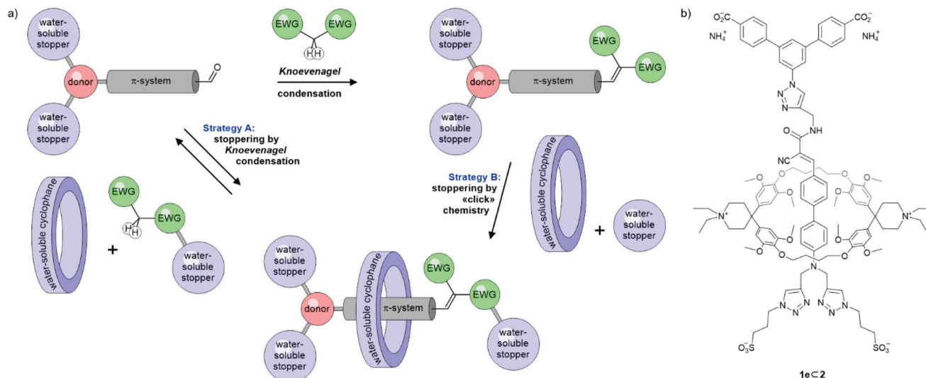
Scheme 1 (a) Both strategies to assemble rotaxanes with a D-π-A chromophore as axis considered. (b) Rotaxane 1e2 obtained via strategy B.
