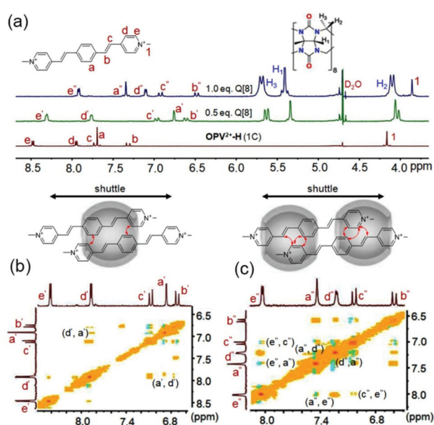
Fig. 2 (a) 1 H NMR spectra of OPV 2+ -H (1C) (1.0 mM in D 2 O) with different concentrations of Q[8] (0–1.0 mM); 1 H– 1 H NOESY of OPV 2+ -H (1C)/Q[8] at molar ratios of 2:1 (b) and 2:2 (c).
