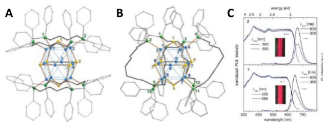
Fig. 7 Molecular structure of (A) [\text{Cu}_{12}\text{S}_6(\text{dppt})_4] and (B) [\text{Cu}_{12}\text{Se}_6(\text{dppt})_4] clusters. Colour codes of the elements: Cu: blue, S: yellow, P: green and C: grey. H atoms are omitted for clarity. (C) Room temperature photoluminescence excitation (PLE) and emission (PL) spectra of a suspension of freshly prepared microcrystals of [\text{Cu}_{12}\text{S}_6(\text{dppt})_4] (down) and [\text{Cu}_{12}\text{Se}_6(\text{dppt})_4] (up) in toluene, measured in the integrating sphere. The inset shows the colours of the suspensions of microcrystal under white LED light. Republished with permission from ref. 164. Copyright 2014 Royal Society of Chemistry.
