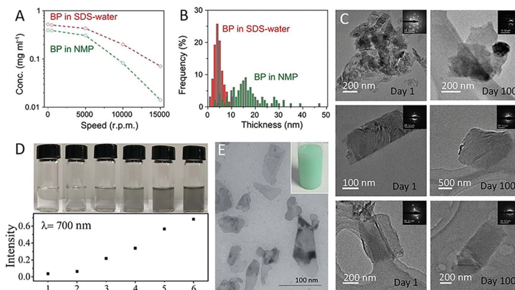
Fig. 8 (A) BP concentration as a function of the centrifugal speed and (B) thickness distribution comparison between BP exfoliated in SDS-water and NMP. (C) PILs-modified PB nanosheet stability for 100 d with TEM monitor. (D) Digital images and absorption intensity of an antimony crystal exfoliated in different systems, 1 to 6 stand for DMF, isopropyl alcohol (IPA), IPA : water (4 : 1), 2-butanol, DMF + P([VPlm]TFSI) and DMF + P([VPlm]PF 6 ), respectively. (E) TEM image of Ni(OH) 2 nanoflakes. Inset: a photo of Ni(OH) 2 dispersion. Reproduced from ref. 188, 196, 202 and 205 with permission from United States National Academy of Sciences, Wiley-VCH and Royal Society of Chemistry.
