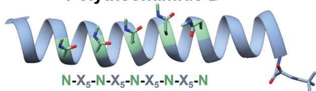
Fig. 2 NMR solution structure of polytheonamide B (PDB: 2RQO) reveals N-methyl Asn are found on one face of the \beta -helix. This repeating N-X 5 -N motif was targeted for genome mining efforts.
