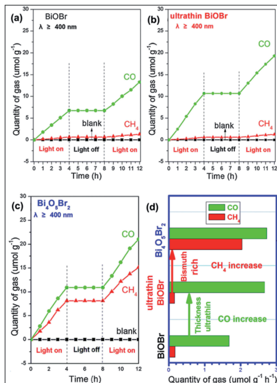
Fig. 7 Photocatalytic reduction performance for the conversion of \text{CO}_2 on (a) \text{BiOBr} ; (b) ultrathin \text{BiOBr} ; and (c) \text{Bi}_4\text{O}_5\text{Br}_2 and (d) comparison of solar fuel generation. Reproduced with permission from ref. 40 Copyright 2016, Elsevier B.V.
