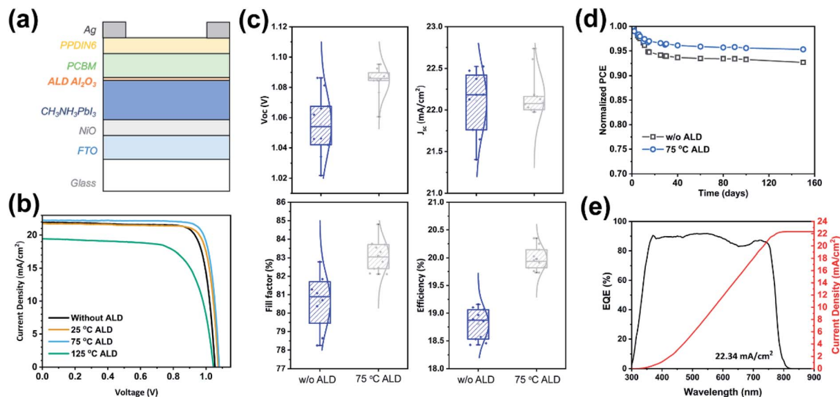
Fig. 3 (a) Schematic architecture of the ambient-prepared PSCs with an ALD \text{Al}_2\text{O}_3 interlayer: FTO/ \text{NiO}_x /MAPbI 3 /ALD- \text{Al}_2\text{O}_3 /PCBM/PPDI6/Ag. (b) Curves of current density versus voltage ( J-V ) for the PSCs with and without 10 cycles of ALD of \text{Al}_2\text{O}_3 deposited at 25 °C, 75 °C and 125 °C, and the corresponding statistical distributions of performance parameters are shown in Fig. S2† (c) Statistical distributions of V_{\text{oc}} , J_{\text{sc}} , fill factor, and PCE for the PSCs with and without ALD \text{Al}_2\text{O}_3 deposited at 75 °C. (d) Long-term stability of PSCs in a \text{N}_2 atmosphere. (e) Incident photon-to-electron conversion efficiency (IPCE) spectrum and the corresponding integrated current density for the PSCs with 10 cycles of ALD of \text{Al}_2\text{O}_3 at 75 °C ((b): 75 °C ALD).
