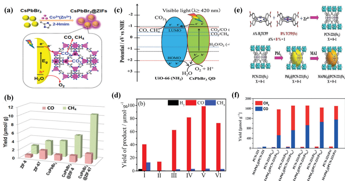
Fig. 13 (a) Schematic illustration of the fabrication process and \text{CO}_2 photoreduction process of \text{CsPbBr}_3 /ZIFs. (b) The product yield after 3 h of photocatalytic reaction. (a and b) Reprinted with permission from ref. 102, Copyright 2018 American Chemical Society. (c) Schematic illustration of a possible mechanism of photocatalytic \text{CO}_2 reduction. (d) Photocatalytic \text{CO}_2 reduction performance for \text{CsPbBr}_3 QDs and \text{x\%-CsPbBr}_3 QDs/ \text{UiO-66}(\text{NH}_2) nanocomposite. (c and d) Reprinted from ref. 113, Copyright (2019), with permission from Elsevier. (e) Schematic representation for the synthesis of \text{PCN-221}(\text{Fe}_x) MOF and \text{MAPbI}_3 @ \text{PCN-221}(\text{Fe}_x) composite photocatalysts for stable and product selective \text{CO}_2 reduction. (f) Histogram of product formation using \text{PCN-221}(\text{Fe}_x) and \text{MAPbI}_3 @ \text{PCN-221}(\text{Fe}_x) . (e and f) Reproduced with permission from ref. 45, Copyright 2019 Wiley.
