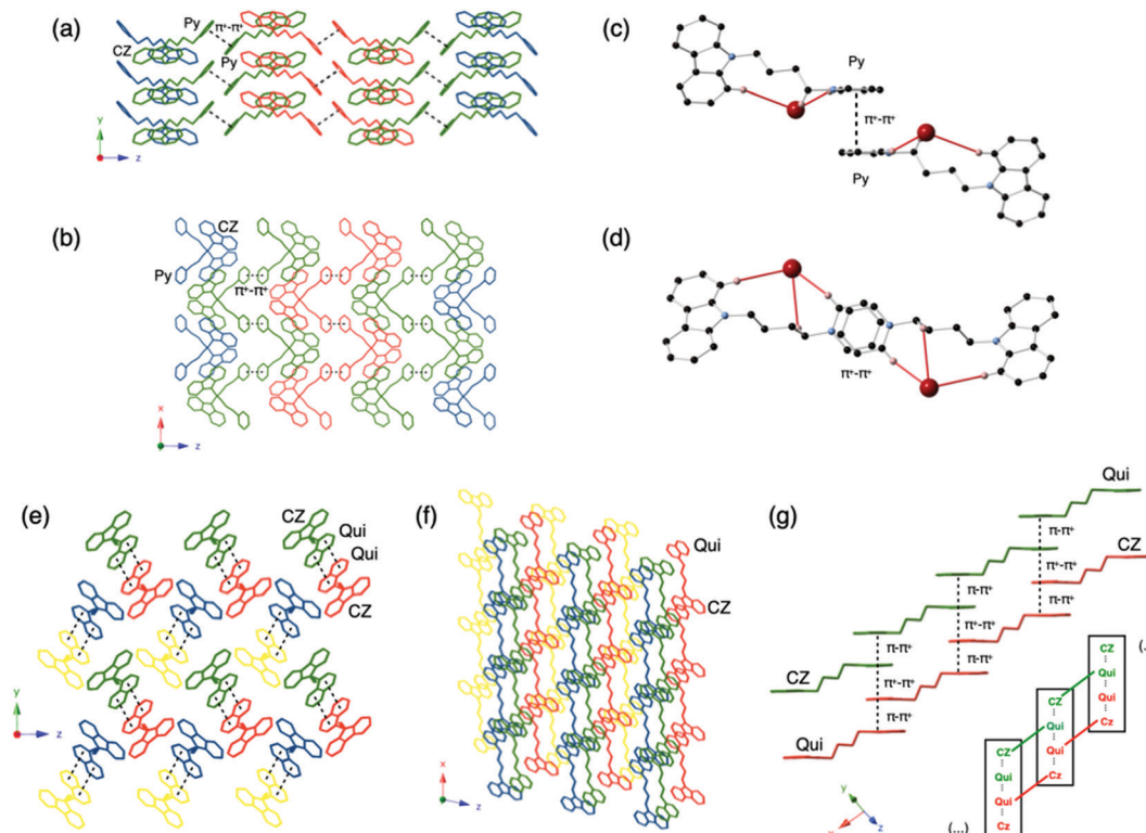
Fig. 1 Different crystal views of the intermolecular packing of Py-Br (a and b) and Qui-Br (e and f). (c and d) Molecular \pi^+ \cdots \pi^+ and \text{Br}-\text{H} interactions in Py-Br . (g) Molecular \pi^+ \cdots \pi^+ and \pi^+ \cdots \pi^+ interactions in Qui-Br .
