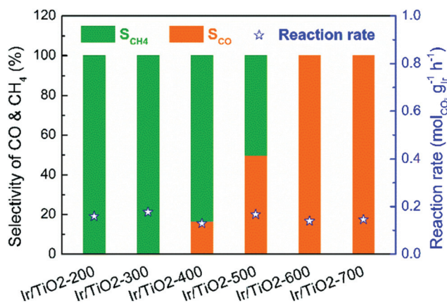
Fig. 9 Catalytic performance of the series of Ir/TiO 2-x catalysts for CO_2 hydrogenation reactions. Reaction conditions: 280 °C, 0.1 MPa, space velocity = 9000 mL h -1 g cat -1 , and H_2/CO_2/N_2 = 70/20/10 . X refers to the reduction temperature in °C. 128
