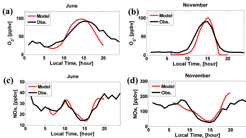
Fig. 2 Observed and simulated ozone and NO x diurnal variations. (a) Ozone in June; (b) ozone in November, (c) NO x in June, and (d) NO x in November. The black line indicates observations and the red line indicates NCAR-MM model results.
