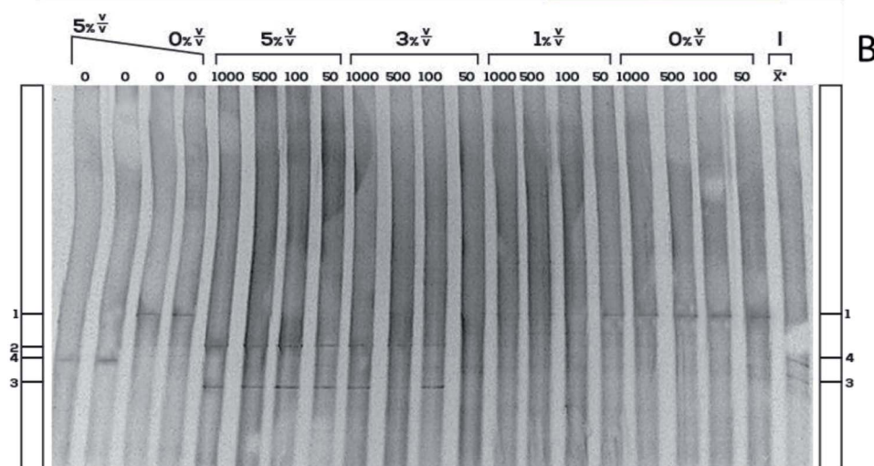
Fig. 3 (A) Maximum likelihood inferred 16S rRNA phylogenetic reconstruction from excised DGGE bands. Black circles correspond to a 1000 bootstrap, SH-aLRT \geq 80\% and ultra-fast bootstrap \geq 95\% . (B) DGGE fingerprinting image from the BMP sludge with anaerobic treatment (0% v/v), microaerobic 1% v/v O_2 , 3% v/v O_2 , 5% v/v O_2 and inoculum (I). Numbers on the top of each column (0, 50, 100, 500 and 1000 ppm) correspond to PDMS concentrations per treatment, \bar{X}^* corresponds to the PDMS concentration inferred from literature. Dominant DGGE bands correspond to the chart at the bottom and the phylogenetic reconstruction.
