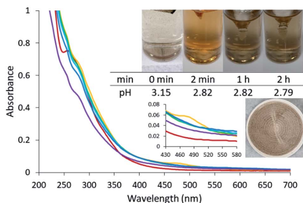
Fig. 20 UV-Vis absorption spectra of mixture of excess Fe(III) and BBOA extracts. Different colors of traces correspond to the spectra of BBOA before mixing (red), 2 min after mixing (orange), 30 min after mixing (green), 1 h after mixing (light blue), 2 h after mixing (dark blue), and filtered solution (purple). Reproduced from ref. 190 under Creative Commons License (CC BY-NC) from the Royal Society of Chemistry, © The Author(s), 2021.
