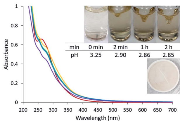
(c) BBOA (Pine #3) + FeCl 3
