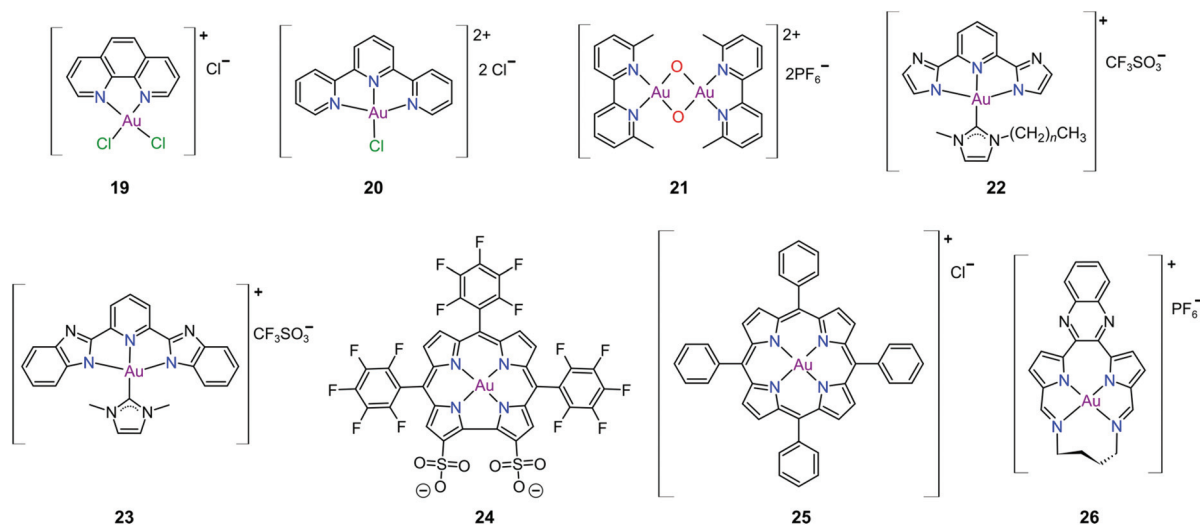
Fig. 12 Representative Au(III) chelates of polydentate N-donor ligands ( 19–23 ), a corrole derivative ( 24 ), a tetra(aryl) porphyrin derivative ( 25 ), and a bis(pyrrolide-imine) macrocycle ( 26 ). Ligands 24–26 effectively stabilize the Au(III) ion against reduction under physiological conditions.
